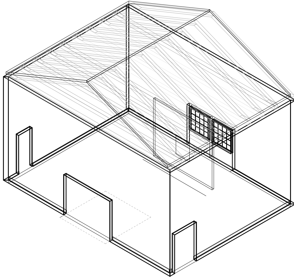
1 Corkran Gallery Right Isometric Scale: 3/16" = 1'-0"
