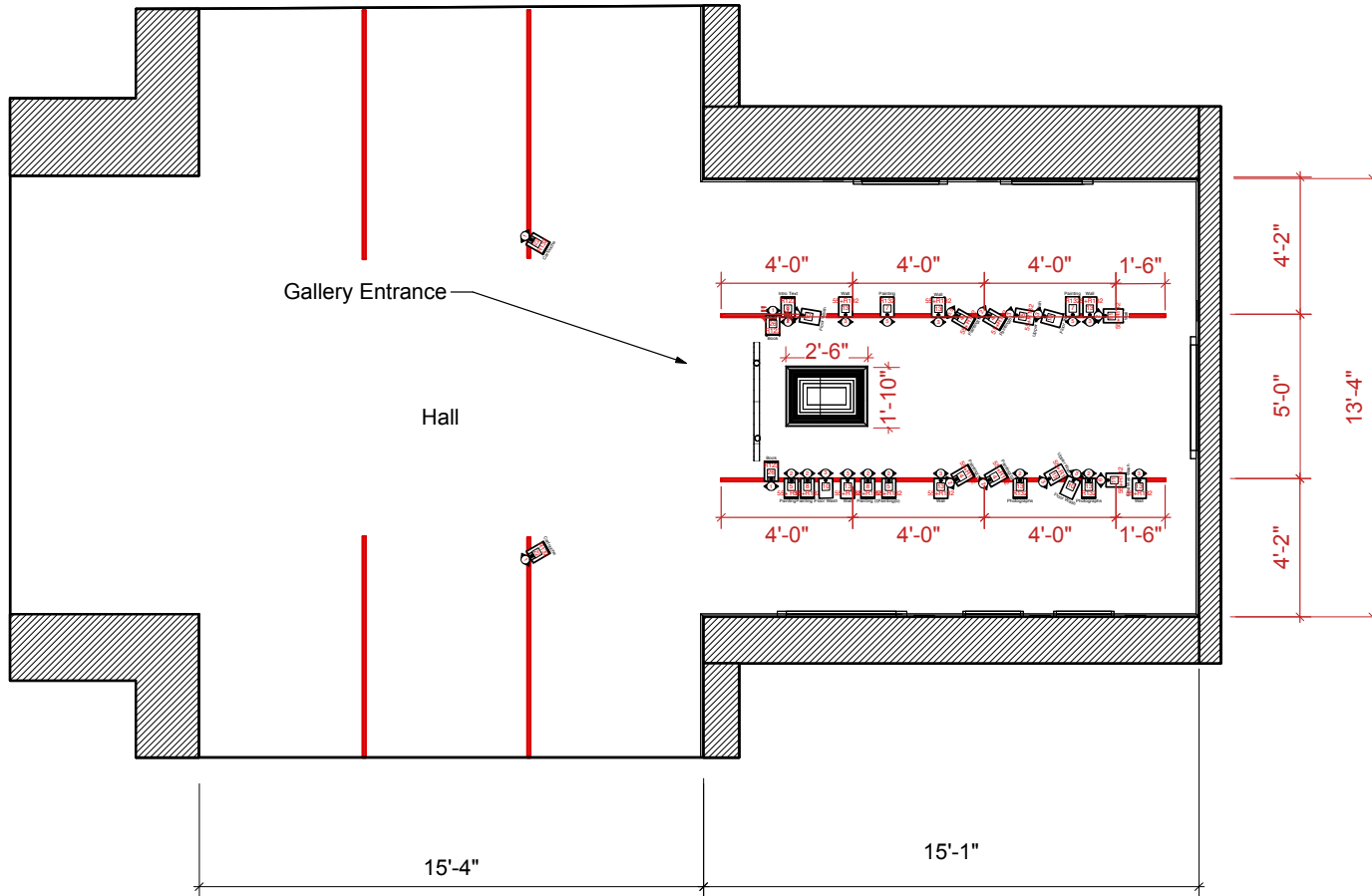
1 Floor plan Sht. 1 Scale: 3/8" = 1'-0"
