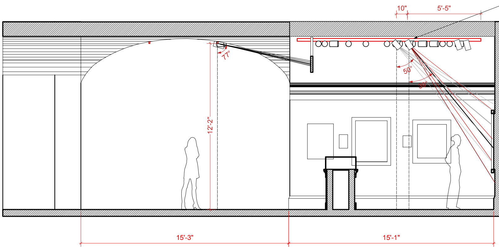
3 EAST/WEST SECTION Sht-4 Scale: 1/2" = 1'-0"
