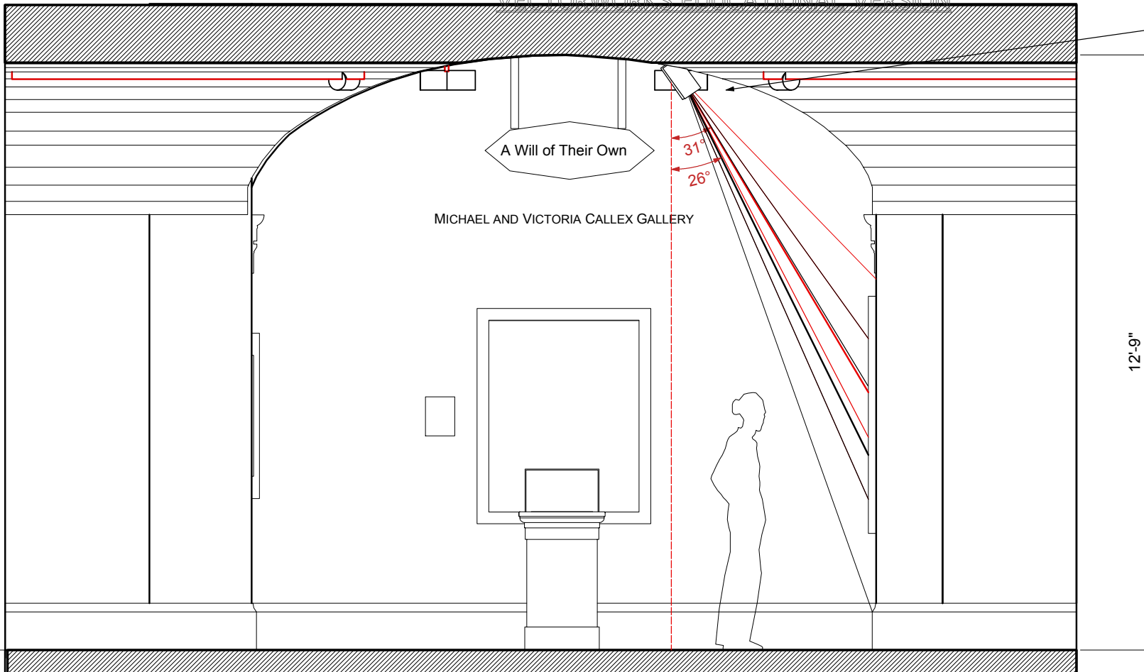
1 NORTH/SOUTH SECTION FACING EAST Sht-2 Scale: 3/4" = 1'-0"
